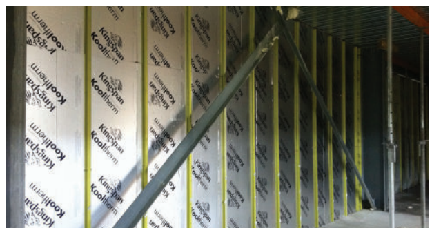
Figure 6 Side elevation of Kingspan Kooltherm ® K12 Framing Board clip-and-channel system
