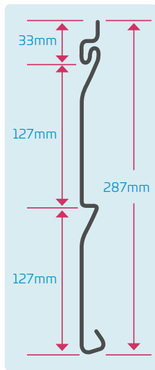
Profile
