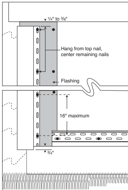
Lapping of outside corner posts
